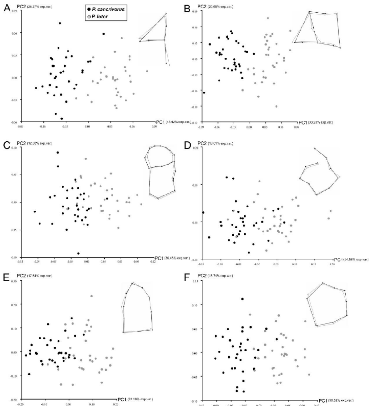
Figure 3 – Scatterplot of shape space defined by first and second principal components; superimposed diagrams illustrate shape differences between species. (A) p4; (C) ml; (E) m2; (B) P4; (D) M1; (F) M2. Percentage of explained variation indicated next to each PC. Black dots and lines: Procyon cancrivorus , gray dots and lines: P. lotor .
