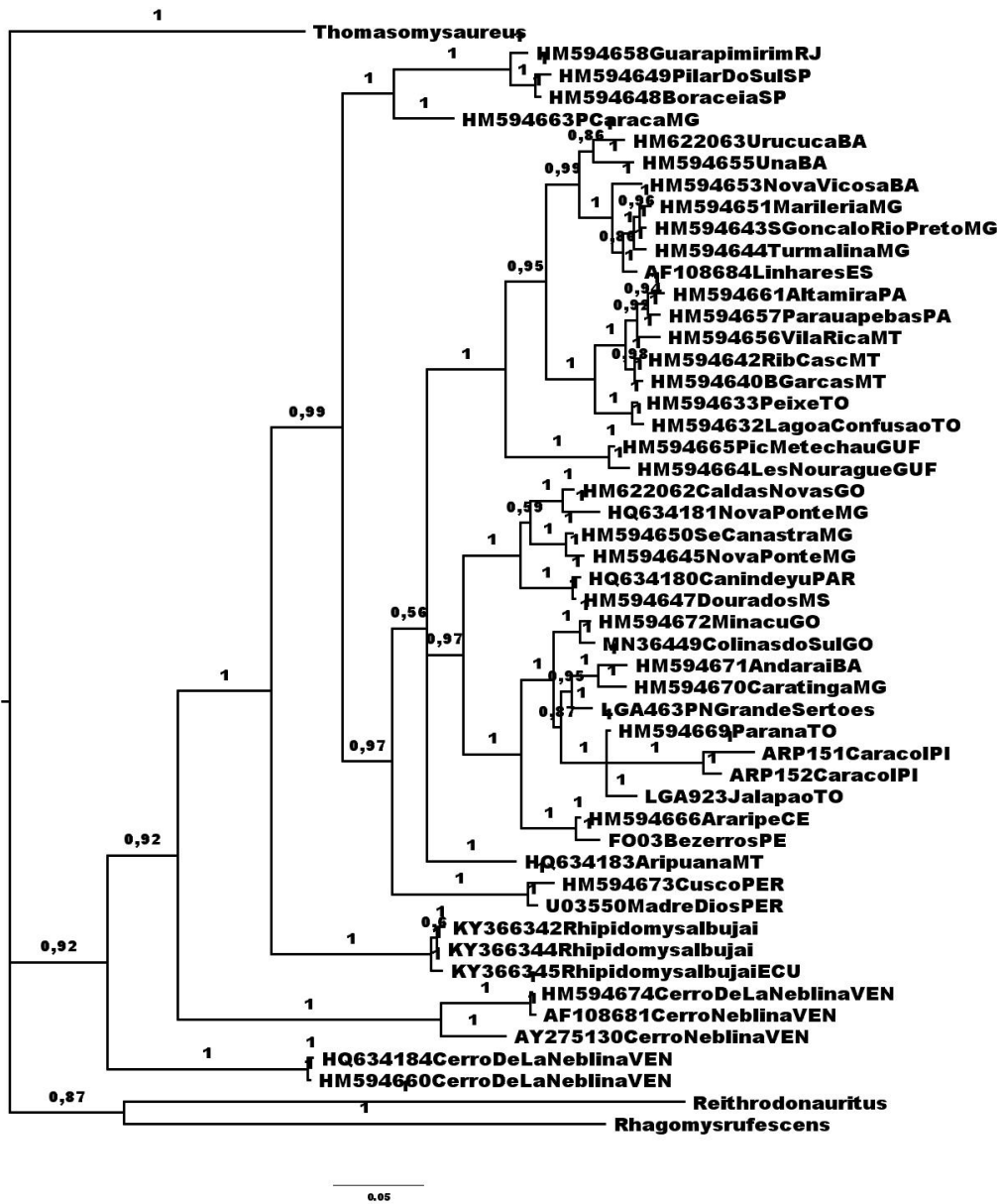
Figure S1. – Bayesian Inference phylogeny. The numbers on the branches corresponds to posterior probability.
